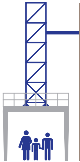
SCAFFOLD GANTRY MAST TIED TO BUILDING
